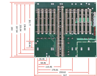
PBP-14PD64 14-slot (8xPCI-X, 4xPCI) 64-bit PICMG 1.2 Backplane - Support 4 independent buses with ROBO-8820VG2H & PA-B1 - Three PCI-X buses; one PCI bus - ATX & aux power connectors support
