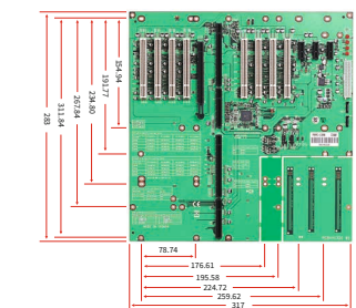
PBPE-13A8 13-slot [PCI (8), PCI-E x16 (1), PCI-E x1 (3)] PICMG 1.3 Backplane - Fit for 4U chassis - Four USB ports - Dual SATA port - 24-pin ESP12V power connector
